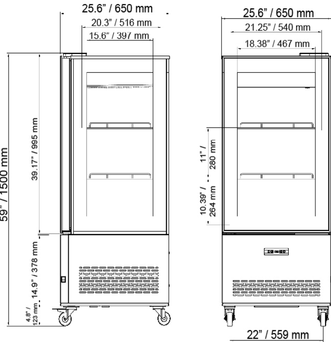
44471 - 26" Wide / 59" Tall
