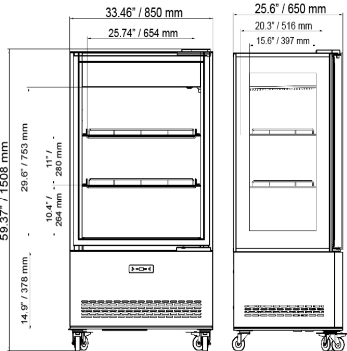
44472 - 33" Wide / 59" Tall
