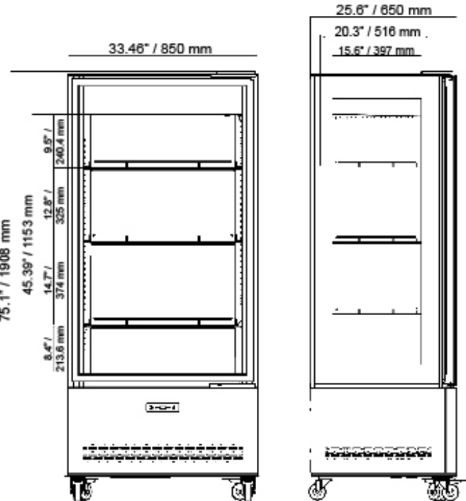
44474 - 33" Wide / 75" Tall
