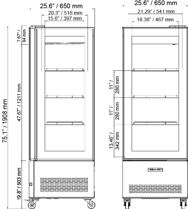
44473 - 26" Wide / 75" Tall
